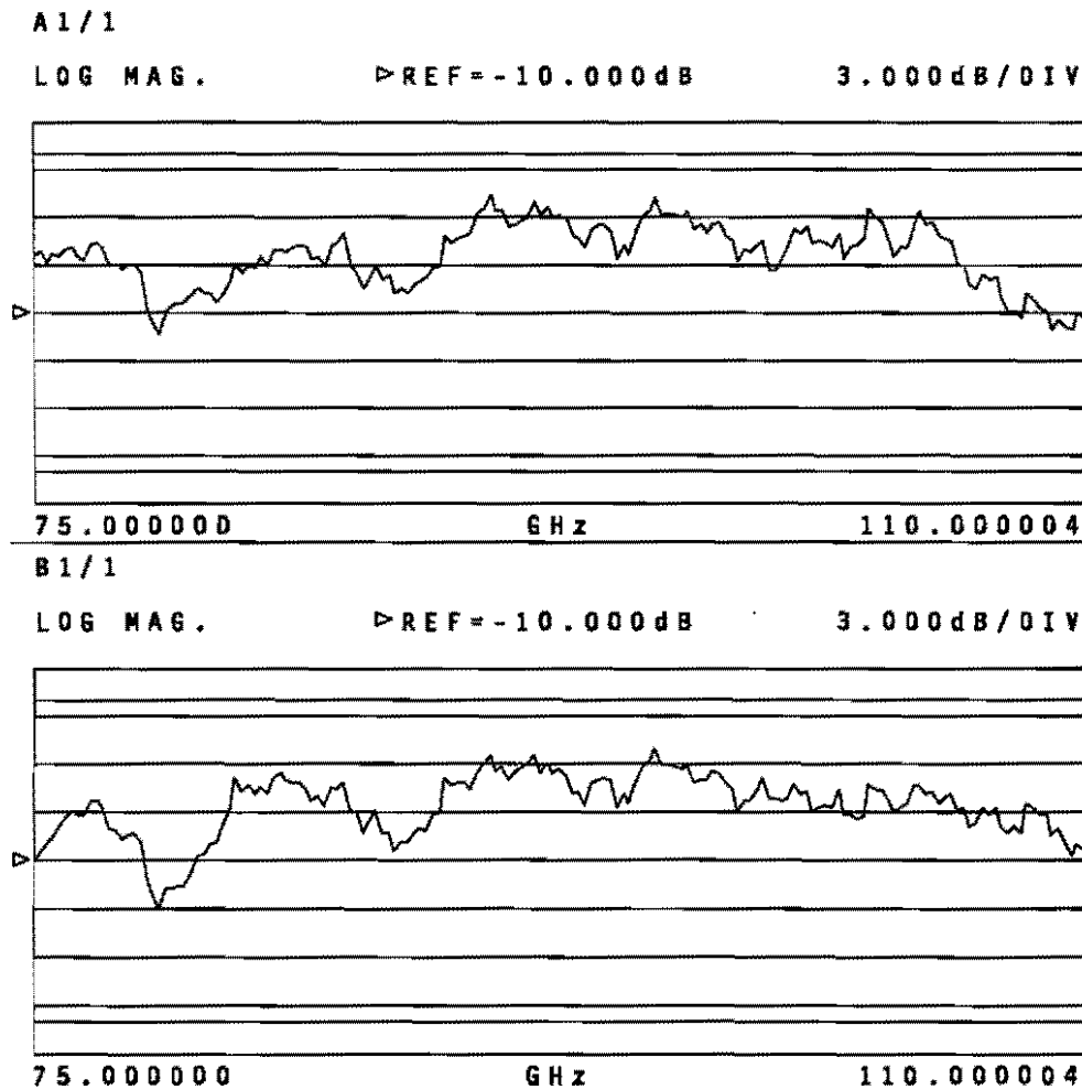
Figure 3-10. Non-Ratioed Power Level Test Dual Channel Waveform for a 3640B-X Module
