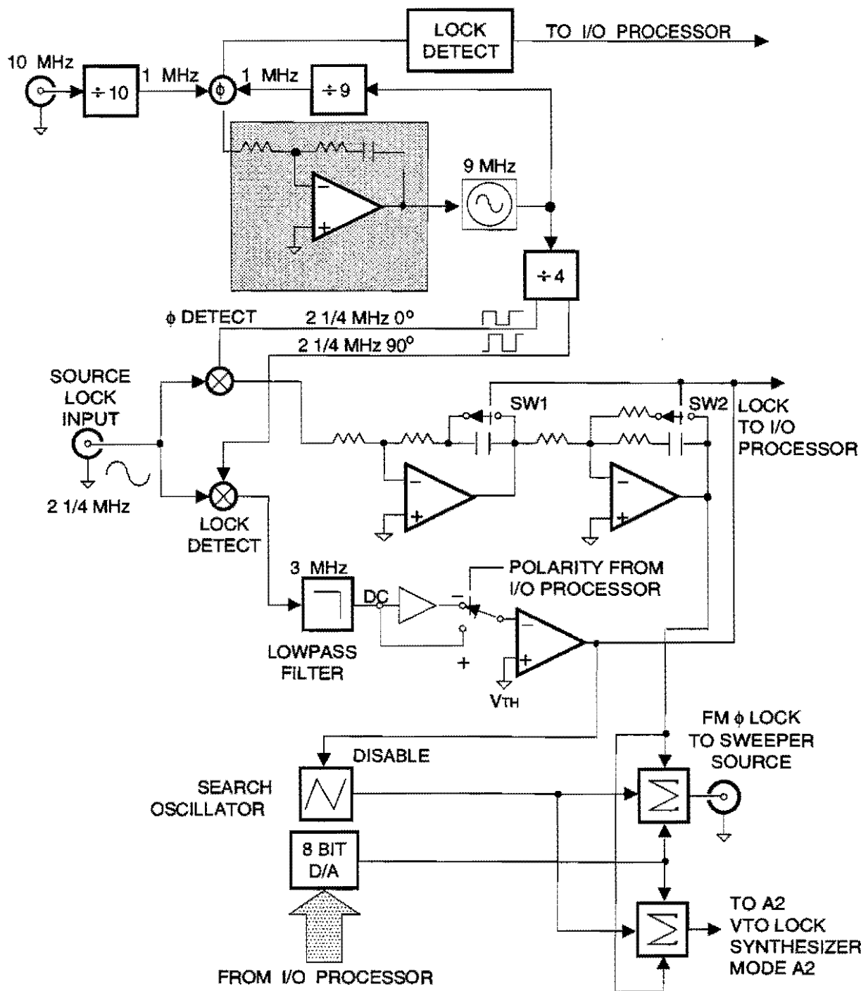
Figure 5-8. A6 Source Lock PCB Block Diagram
