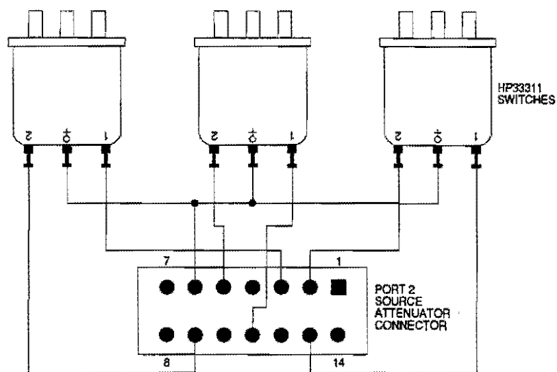
Figure A-6. Port 2 Source Attenuator Connector Controlling Three HP33311 Switches
